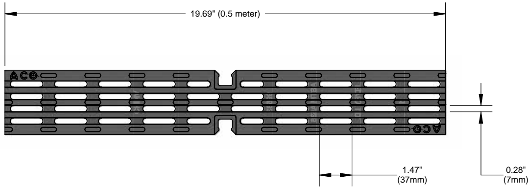
Plan view
