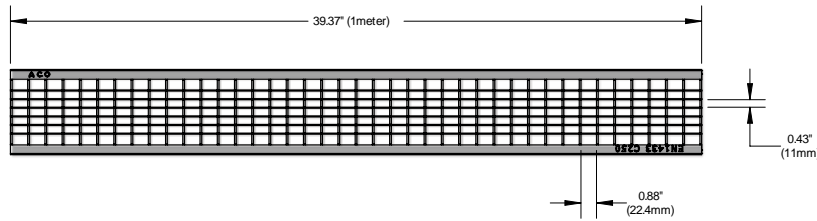
Plan view
