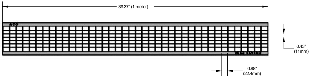
Plan view
