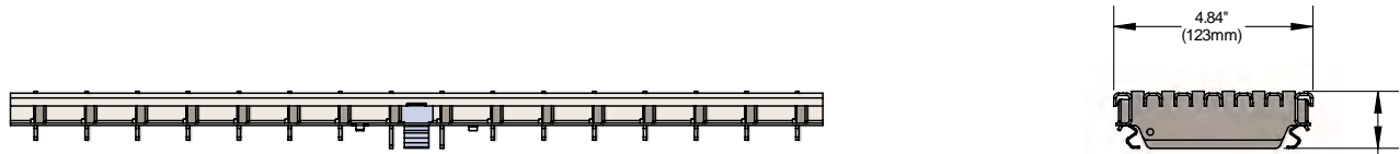
Side elevation
