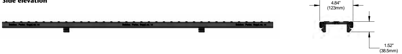
Side elevation
