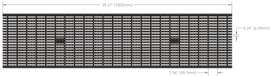
Plan view
